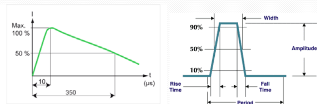
Fig. J9 - 10/350 μs current wave
