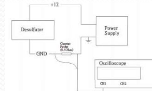
Figure 2-2: Test the prototype circuit with power supply
