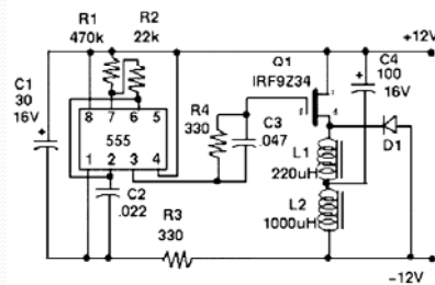
Figure 1: 12 Volt Battery Desulfator
