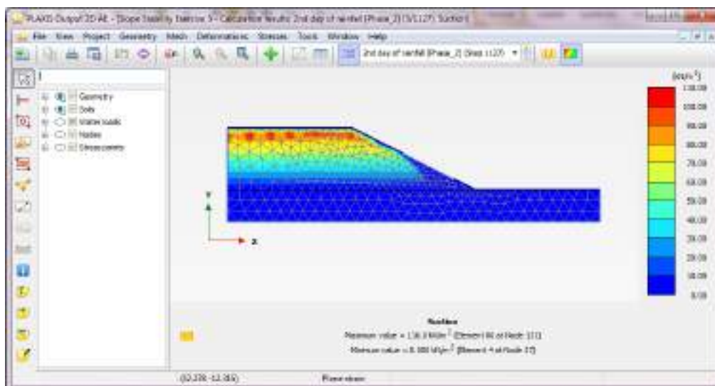
Figure 42: Suction after 2 nd day of rainfall
