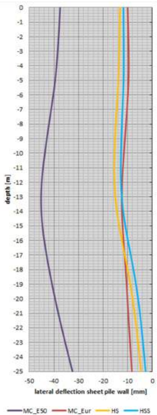
Figure 10: lateral deflection of the sheet pile wall after the last excavation step [mm]
