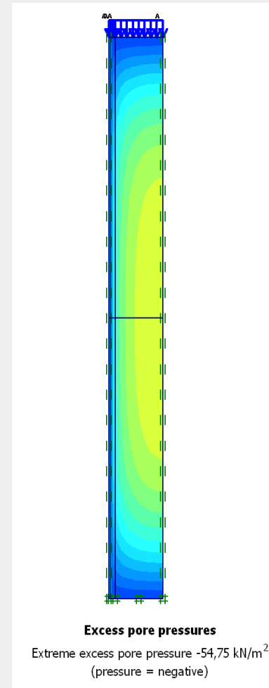
With PVD and Smear Zone
