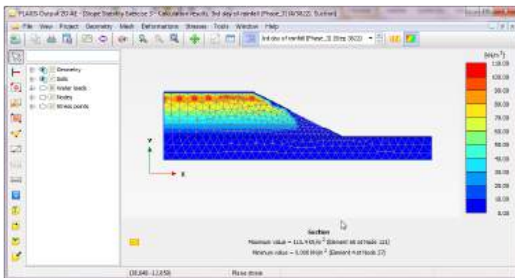
Figure 43: Suction after 3 rd day of rainfall
