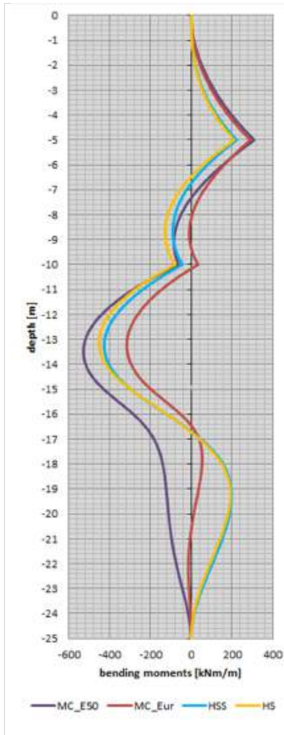
Figure 9: Bending moments after the last excavation step [kNm/m]
