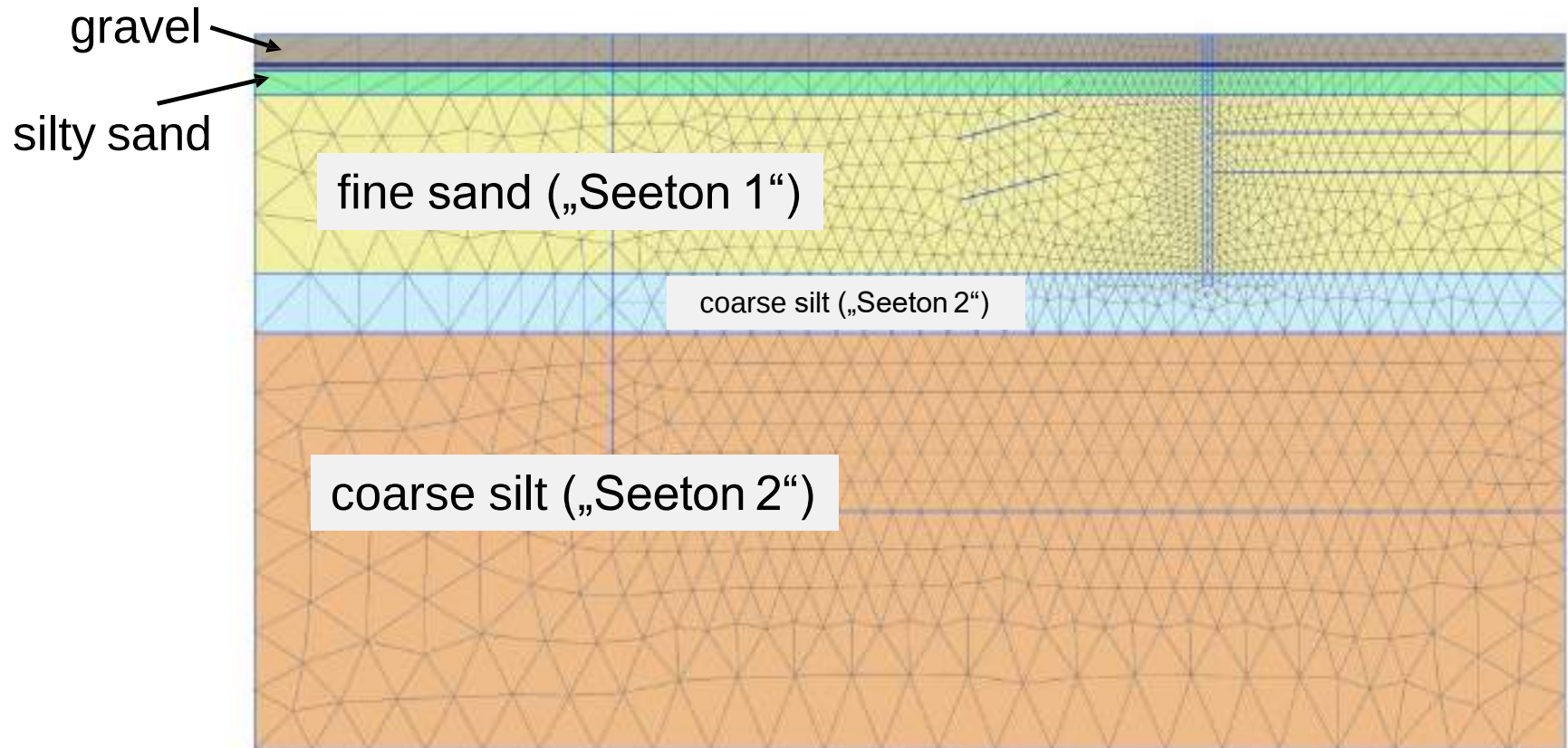
Soil layers and mesh for project „Kiesel“
