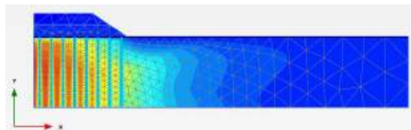
Figure 20: excess pore pressure ( P_{excess} ) with PVD
