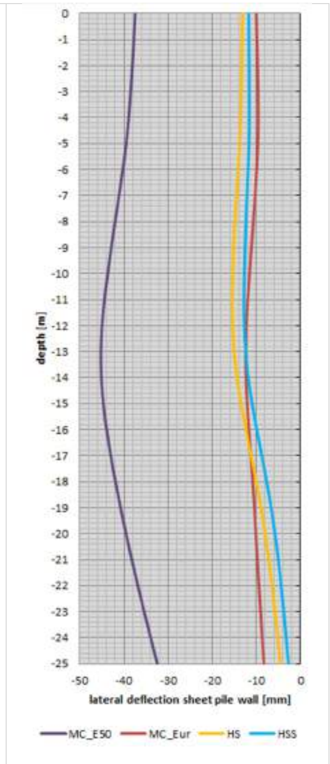
Figure 10: lateral deflection of the sheet pile wall after the last excavation step [mm]
