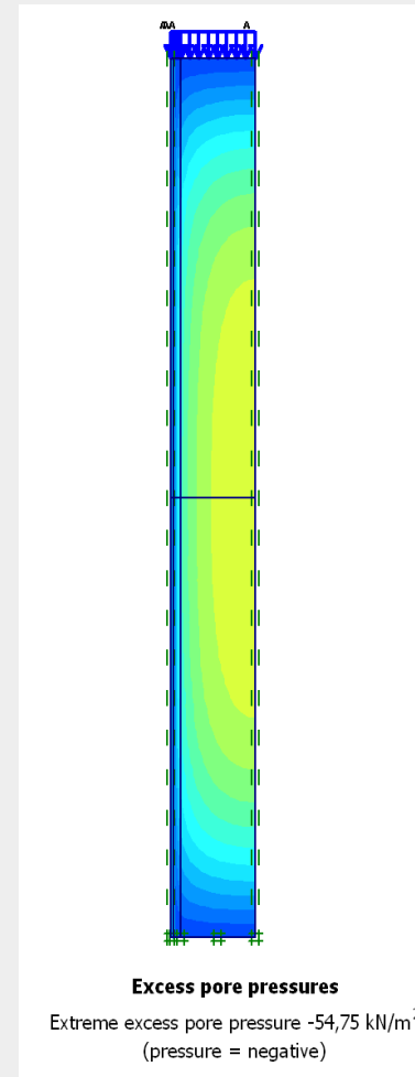
With PVD and Smear Zone
