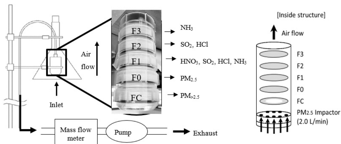
Figure A2. Schematic diagram of a five-stage filter pack sampler. A PM_{2.5} impactor is installed at the sampling inlet to separate coarse ( PM > 2.5 \mu m ) and fine ( PM \leq 2.5 \mu m ) particles. A doughnut shaped filter is used for collection of coarse particles. Fine particulate is passed through the center of the stage FC and collected on the F0 filter [32].
