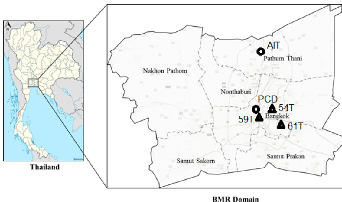
Figure A1. Map of the locations of PM_{2.5} monitoring stations in Bangkok Metropolitan Region having the monthly levels presented in Figure 1. Note: AIT: JICA sites: Asian Institute of Technology (AIT), and Pollution Control Department (PCD). PCD automatic monitoring stations: 54T (Din Daeng), 59T (Government public relation department), and 61T (Bodindecha).
