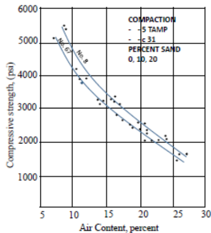
Fig. 1. Air content versus compressive strength at 28-days [3].
