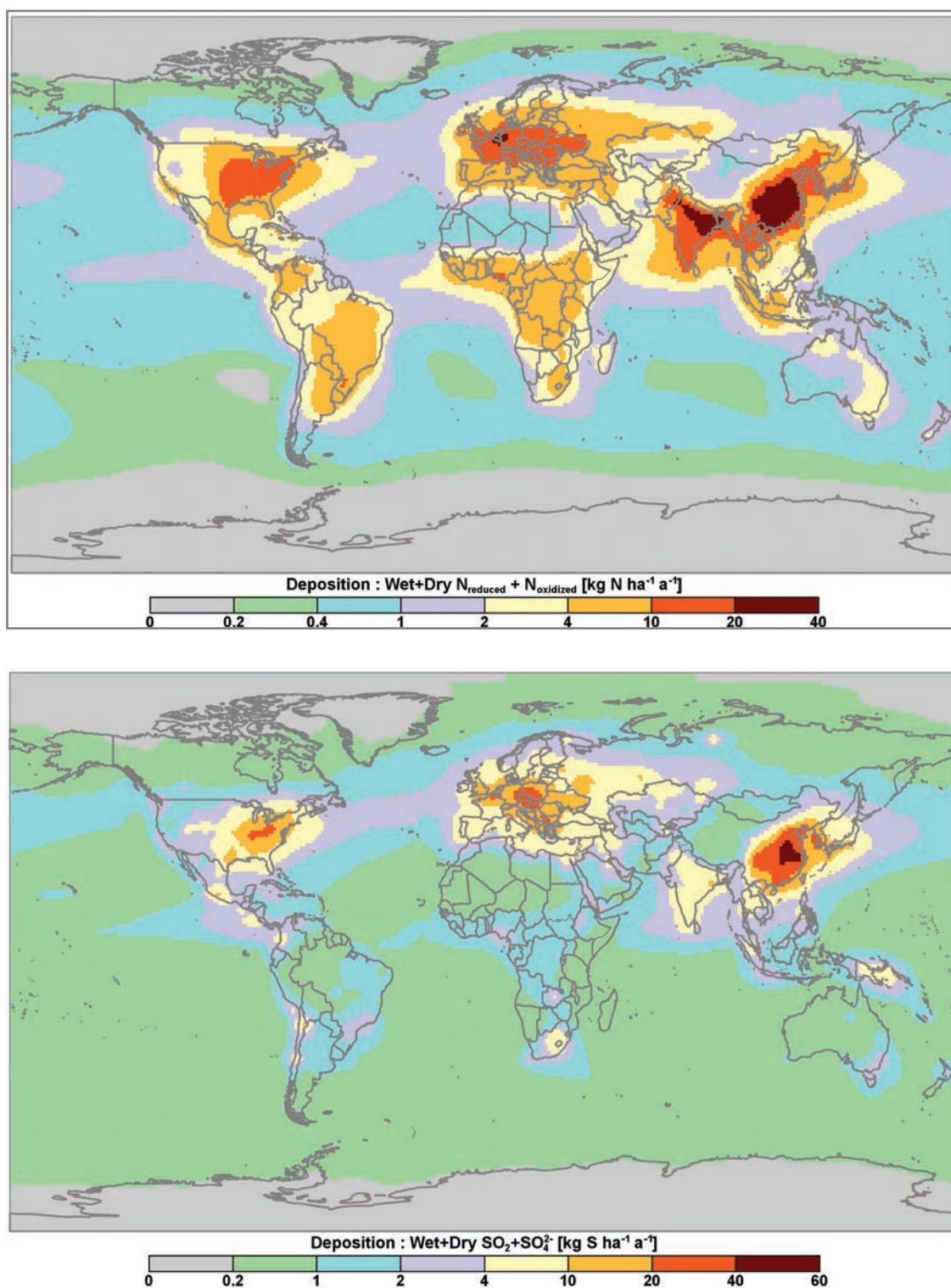
FIGURE 1.14: 2001 ENSEMBLE-MEAN PATTERNS OF NITROGEN WET AND DRY DEPOSITION OF OXIDIZED (E.G. NITRATES AND NO x ) AND REDUCED (E.G. AMMONIUM AND AMMONIA) FORMS (ABOVE) AND SULPHUR WET AND DRY DEPOSITION (E.G. SULPHATE AND SULPHUR DIOXIDE) (BELOW)
